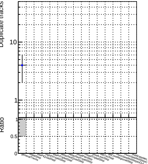
Number Q0M_V0001_R0000000001 Global CMSSW_mkfitt10mu_LowptQ_RECO Q0M_V0001_R0000000001 Global CMSSW_mkfitt10mu_LowptQnoBKW_RECO
