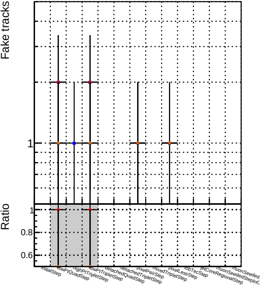
Number ★ DQM_V0001_R000000001 Global CMSSW_mkfit10mu_LowptQ_RECO ★ DQM_V0001_R000000001 Global CMSSW_mkfit10mu_LowptQnoBKW_RECO
