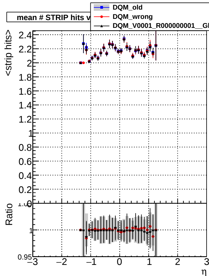
Global_CMSSW_X_Y_Z_RECO
