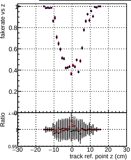
Fake rate vs track ref. point z (cm) Legend: DQM_old (blue), DQM_wrong (red), DQM_V0001 (black) Global CMSSW X Y Z RECO
