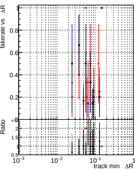
Fake rate vs \Delta R(\text{track, jet}) DOM_old DOM_wrong DOM_V0001_R000000001 Global CMSSW X Y Z RECO
