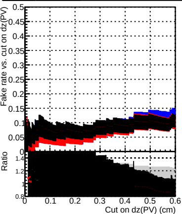
Fake rate vs. cut on dz(PV) (cm)
