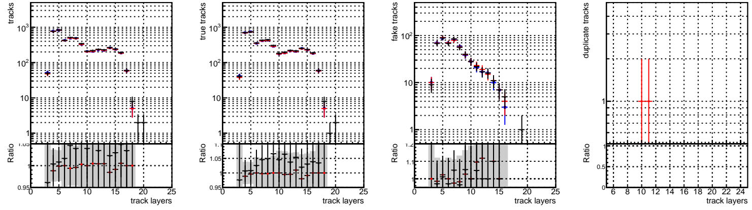
N of reco track vs R00000001 Global CMSSW X Y Z RECO
