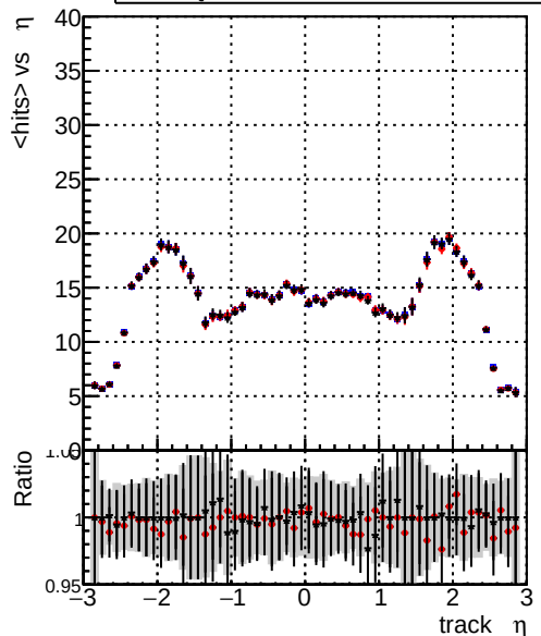
mean hits vs \eta — DQM_old — DQM_wrong — DQM_V0001_R000000001_Global_CMSSW_X_Y_Z_RECO
