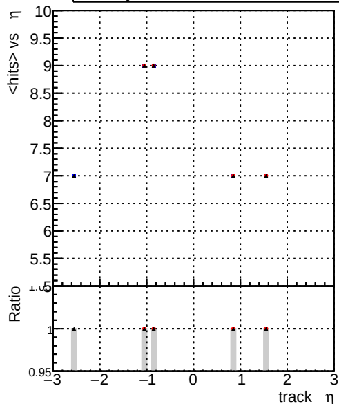
mean hits vs track \eta
