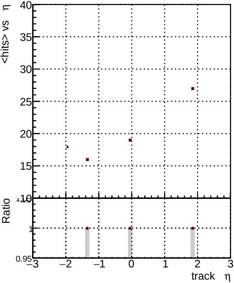
mean hits vs \eta Legend: DQM_old (blue), DQM_wrong (red), DQM_V0001 (black) Global_CMSSW_X_Y_Z_RECO
