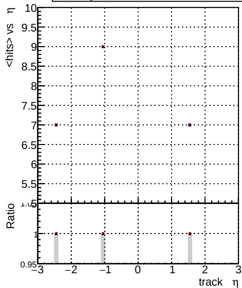
mean hits vs \eta Legend: DQM_old (blue), DQM_wrong (red), DQM_V0001 (black) mean hits: R000000001_Global_CMSSW_X_Y_Z_RECO
