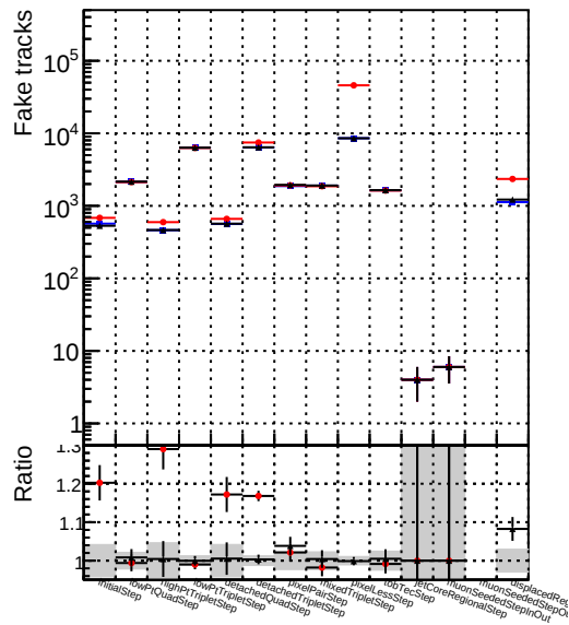
Number of tracks vs collection Legend: DQM_old DQM_wrong DQM_V0001
