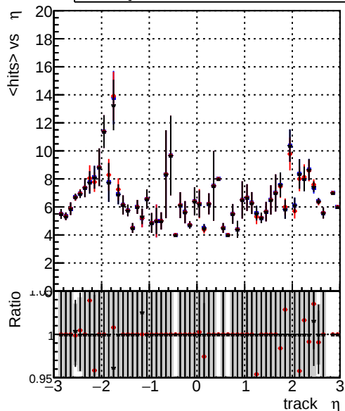
mean hits vs \eta — DQM_old — DQM_wrong — DQM_V0001_R000000001_Global_CMSSW_X_Y_Z_RECO
