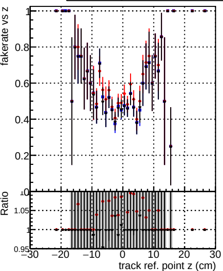
Fake rate vs verpos Global CMSSW X Y Z RECO
