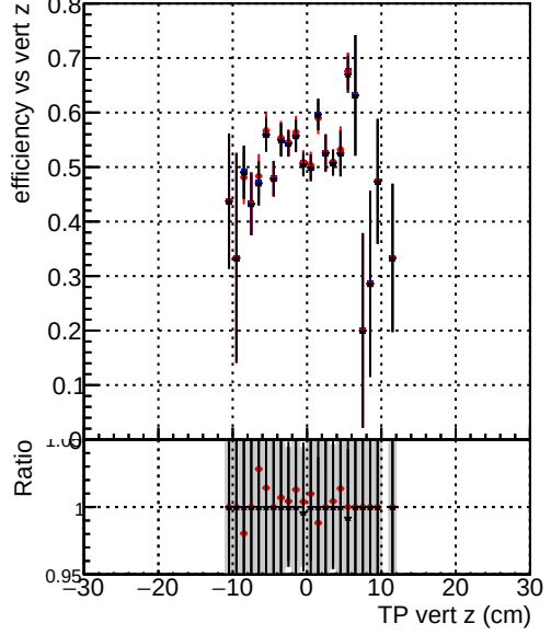
Efficiency — DQM_old — DQM_wrong — DQM_V0001_R000000001_Global_CMSSW_X_Y_Z_RECO
