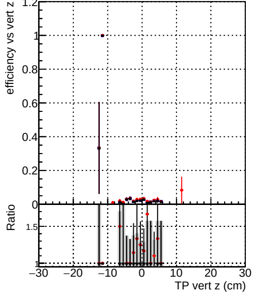
Efficiency vs vert z Legend: DQM_old (blue), DQM_wrong (red), DQM_V0001 (black), R000000001 (grey), Global (black), CMSSW_X_Y_Z (black), RECO (black)
