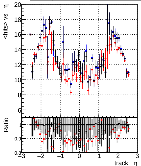
mean hits vs \eta Legend: DQM_old (blue line), DQM_wrong (red line), DQM_V0001_R000000001_Global_CMSSW_X_Y_Z_RECO (black line)
