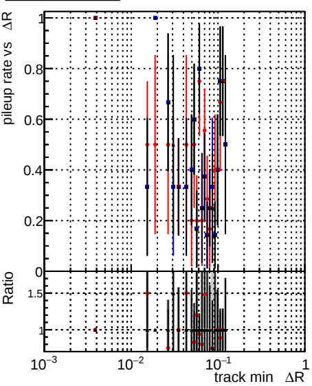
Fake rate vs \Delta R(\text{track, jet}) Duplicates Rate vs \Delta R(\text{track, jet}) Pileup rate vs \Delta R(\text{track, jet}) Global CMSSW X Y Z RECO
