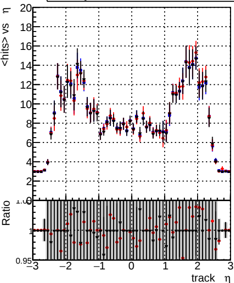
mean hits vs \eta — DQM_old — DQM_wrong — DQM_V0001_R000000001_Global_CMSSW_X_Y_Z_RECO
