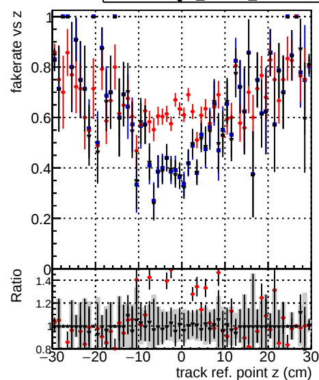
— DQM_old — DQM_wrong — DQM_V0001_R000000001 Fake rate vs track ref. point z (cm)
