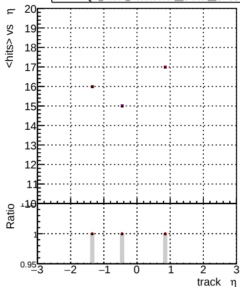
mean hits Legend: DQM_old (blue line), DQM_wrong (red line), DQM_V0001_R000000001_Global_CMSSW_X_Y_Z_RECO (black line)
