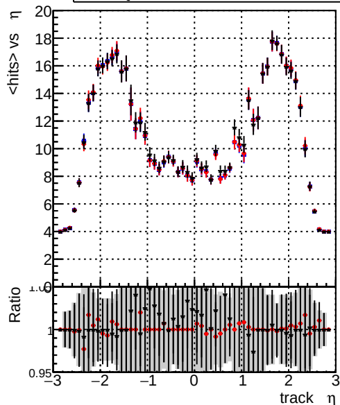
mean hits vs \eta Legend: DQM_old (blue line), DQM_wrong (red line), DQM_V0001 (black line) Global_CMSSW_X_Y_Z_RECO
