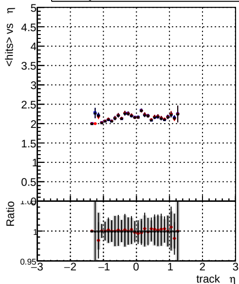
mean hits vs \eta Legend: DQM_old (blue), DQM_wrong (red), DQM_V0001 (black) Global_CMSSW_X_Y_Z_RECO
