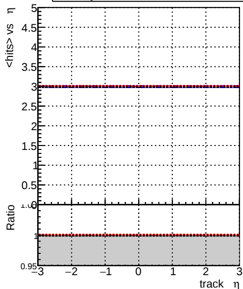
mean hits — DQM_old — DQM_wrong — DQM_V0001_R000000001_Global_CMSSW_X_Y_Z_RECO
