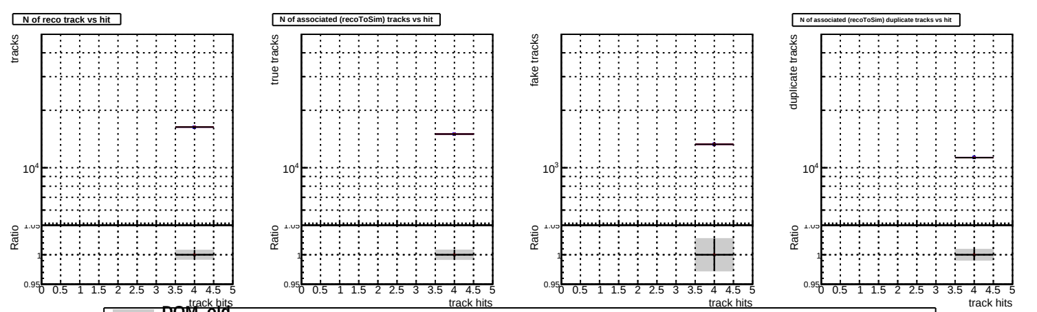
N of reco track vs R000000001 Global CMSSW X Y Z RECO
