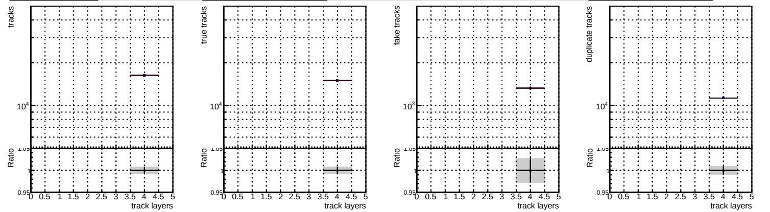
N of reco track vs R000000001 Global CMSSW X Y Z RECO
