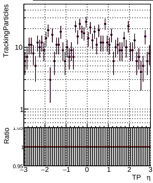
N of simulated tracks vs \eta Legend: DQM_old (blue line with circles), DQM_wrong (red line with circles), DQM_V0001 (black line with circles). The text 'R000000001_Global_CMSSW_X_Y_Z_RECO' is also present.
