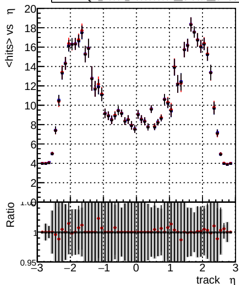
mean hits vs \eta Legend: DQM_old (blue line), DQM_wrong (red line), DQM_V0001_R000000001_Global_CMSSW_X_Y_Z_RECO (black line)
