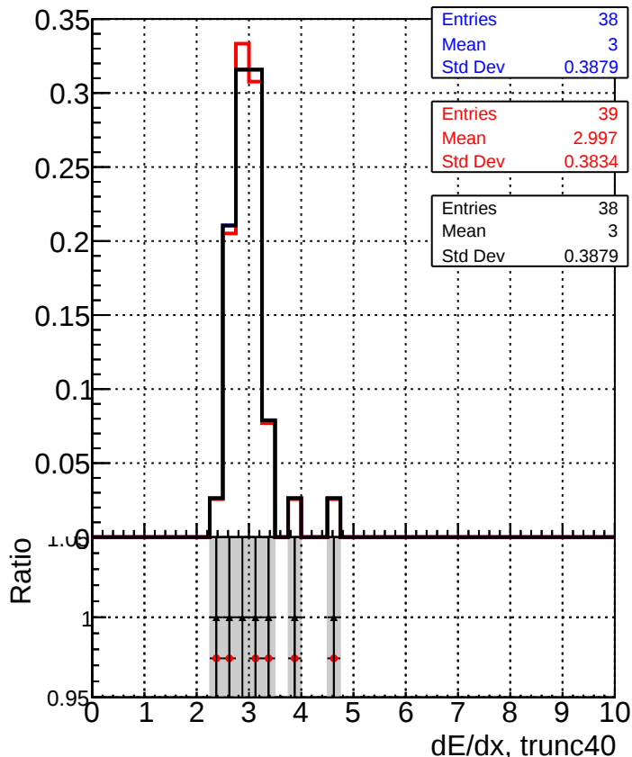
—●— DQM_old —●— DQM_wrong —●— DQM_V0001_R000000001_Global_CMSSW_X_Y_Z_RECO
