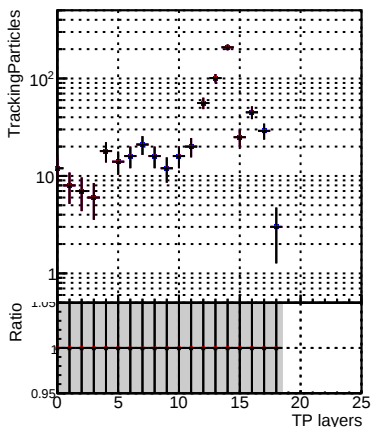
N of sim → DQM_V0001_R000
