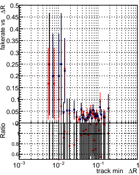
■ DQM_old ● DQM_wrong ▲ DQM_V0001 Fake rate vs \Delta R (track, jet) Global CMSSW X Y Z RECO
