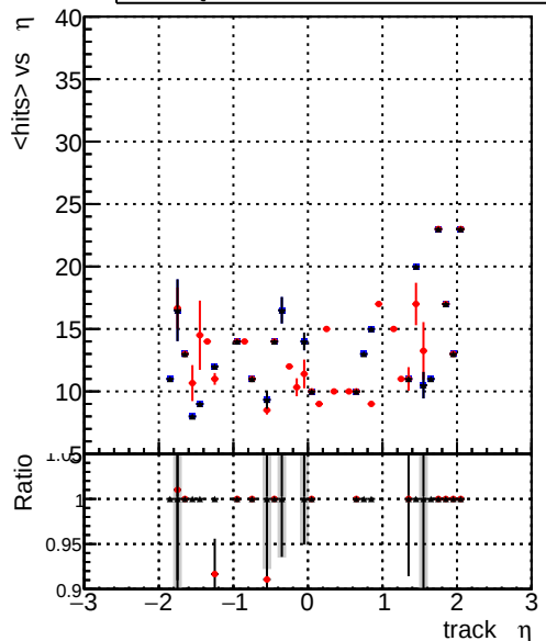
mean hits — DQM_old — DQM_wrong — DQM_V0001_R000000001_Global_CMSSW_X_Y_Z_RECO
