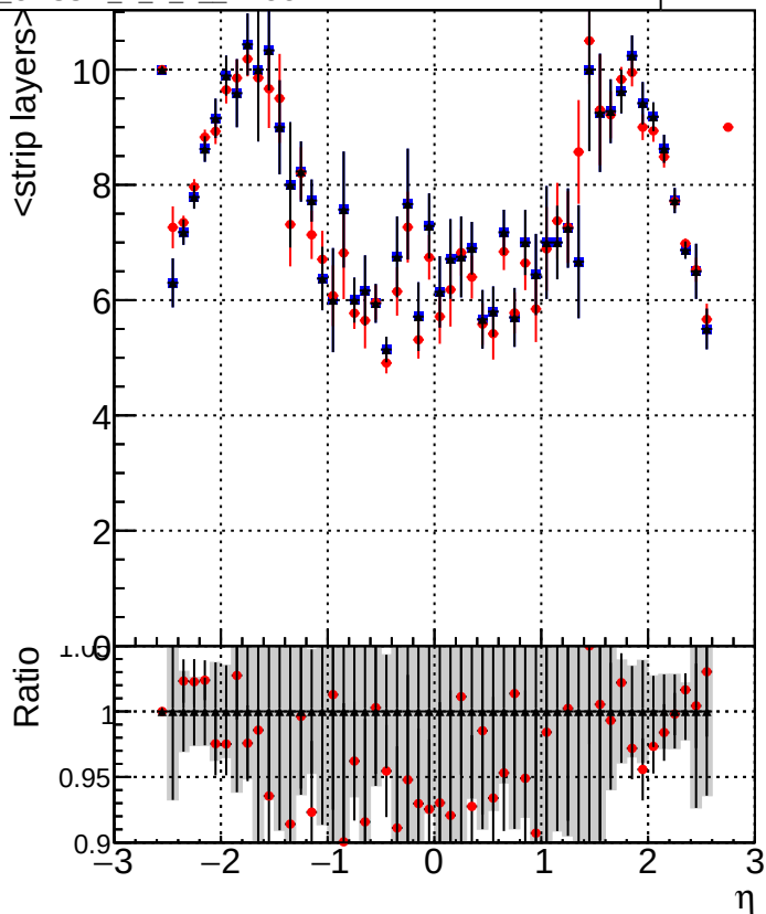
Global_CMSSW_X_Y_Z_RECO
