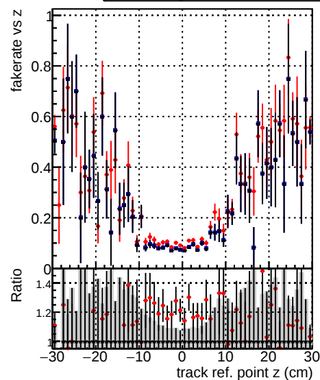
Fake rate vs track ref. point z (cm) Duplicates Rate vs track ref. point z (cm) Pileup rate vs track ref. point z (cm) DOM_old (blue circles) DOM_wrong (red circles) DOM_V0001_R000000001 (black circles) Global_CMSSW_X_Y_Z_RECO
