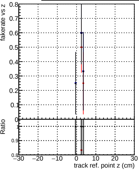
Fake rate vs vertpos Global CMSSW X Y Z RECO
