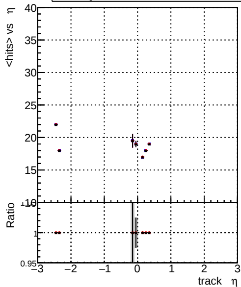
mean hits vs \eta Legend: DQM_old (blue), DQM_wrong (red), DQM_V0001_R000000001_Global_CMSSW_X_Y_Z_RECO (black)
