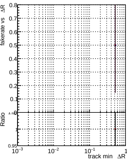
Fake rate vs ΔR(track, jet) Global CMSSW X Y Z RECO
