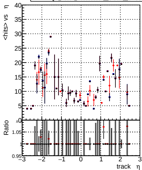
mean hits — DQM_old — DQM_wrong — DQM_V0001_R000000001_Global_CMSSW_X_Y_Z_RECO
