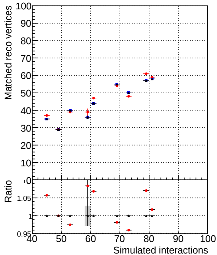
MatchedRecoVtx_vs_GenVtx
