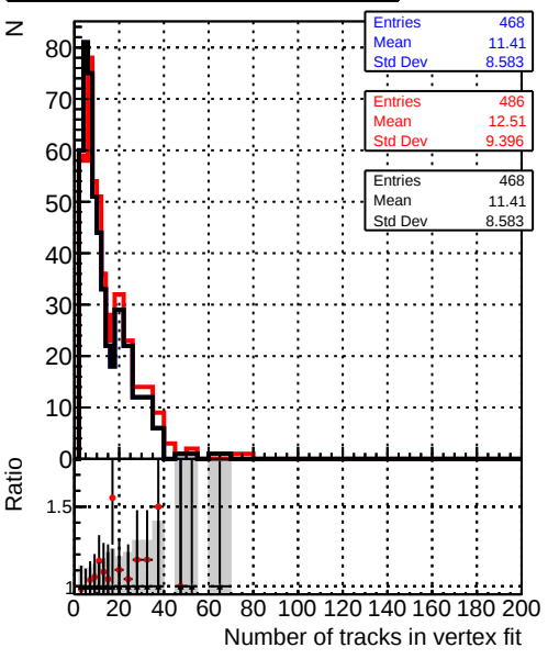
ReconstructedAllAssoc2Gen_NumTracks
