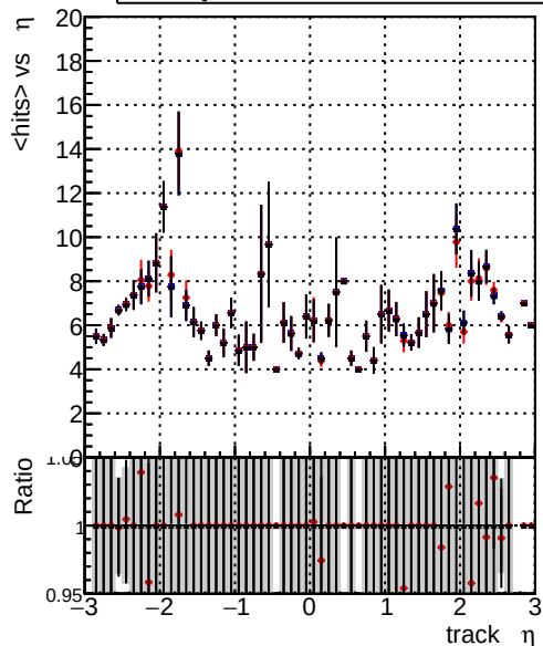
mean hits vs \eta Legend: DQM_old (blue line), DQM_wrong (red line), DQM_V0001 (black line) Global_CMSSW_X_Y_Z_RECO
