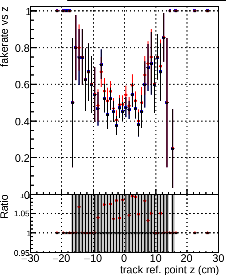
Fake rate vs verpos DOM_old DOM_wrong DOM_V0001 R000000001 Global CMSSW X Y Z RECO
