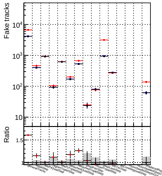
Number of tracks vs collection Legend: DQM_old (blue circles) DQM_wrong (red circles) DQM_V0001_R000000001_Global_CMSSW_X_Y_Z_RECO (black circles)
