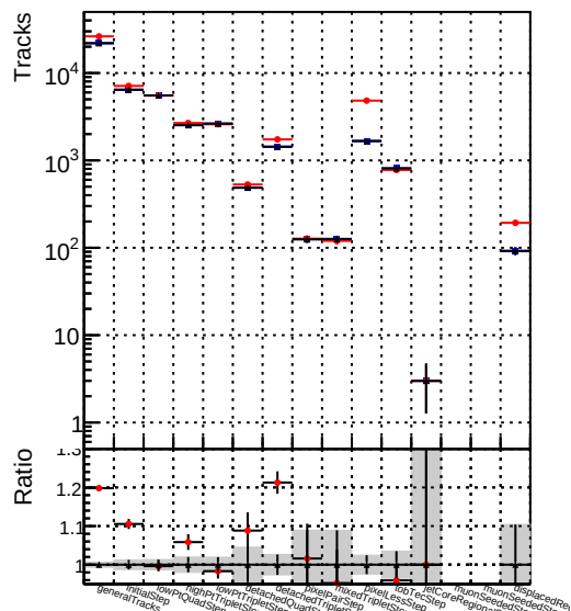
Number of tracks vs collection Legend: DQM_old (blue circles) DQM_wrong (red circles) DQM_V0001_R000000001_Global_CMSSW_X_Y_Z_RECO (black circles)
