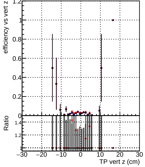
Efficiency vs vert z Legend: DQM_old (blue circles), DQM_wrong (red circles), DQM_V0001 (black circles), R000000001 (grey circles), Global_CMSSW_X_Y_Z_RECO (black line)
