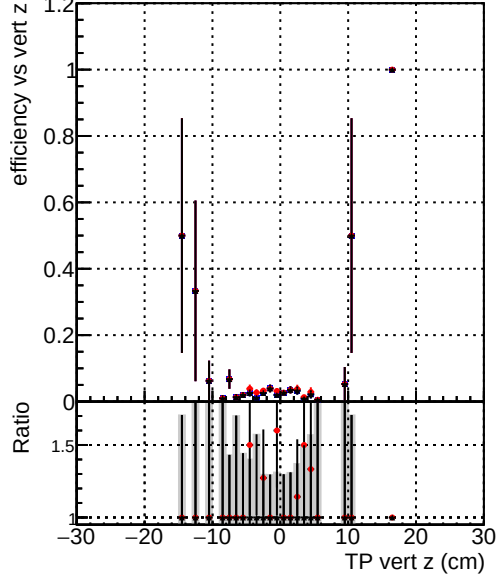
Efficiency vs vert z Legend: DQM_old (blue circles), DQM_wrong (red circles), DQM_V0001 (black circles). Global_CMSSW_X_Y_Z_RECO (grey histogram).
