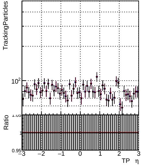
N of simulated tracks vs eta Legend: DQM_old (blue line with circles), DQM_wrong (red line with circles), DQM_V0001 (black line with circles). The legend also includes R000000001_Global_CMSSW_X_Y_Z_RECO.
