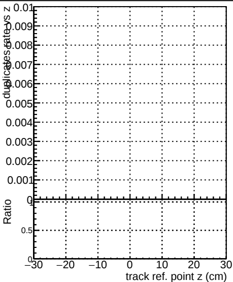
Fake rate vs track ref. point z (cm) Duplicates Rate vs track ref. point z (cm) Pileup rate vs track ref. point z (cm) Global CMSSW X Y Z RECO
