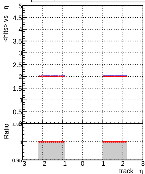
mean hits vs \eta Legend: DQM_old (blue line), DQM_V0001_R000000001_Global_CMSSW_X_Y_Z_RECO (red line)
