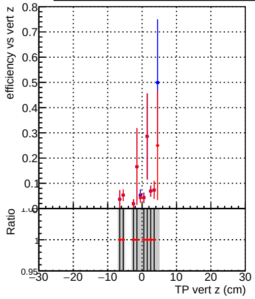
Efficiency vs TP vert z Legend: DQM_old (blue line), DQM_V0001_R000000001_Global_CMSSW_X_Y_Z_RECO (red line)
