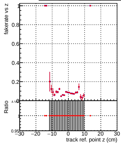
—●— DQM_old —●— DQM_V0001_R000000001_Global_CMSSW_X_Y_Z_RECO
