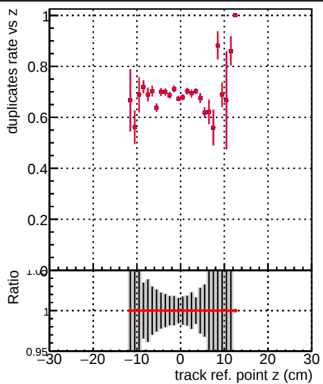
—●— DQM_old —●— DQM_V0001_R000000001_Global_CMSSW_X_Y_Z_RECO
