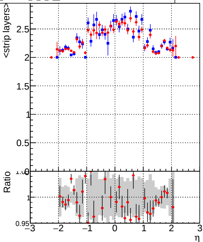
■ DQM_old ● DQM_V0001_R000000001_Global_CMSSW_X_Y_Z_RECO
